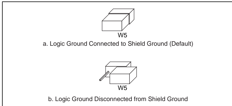
Figure 2-11. AT-GPIB/TNT Ground Configuration Jumper Settings
